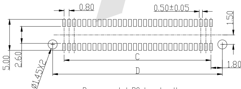
Recommended PC board pattern (TOP VIEW)
